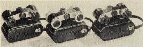
Hensoldt Diadem 2 1/2 x 30, central focusing theatre glass in wide range of colors and finishes, with bending bridge for interpupillary distance setting.
