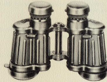
Hensoldt Special Rubber Armored binocular, 8x30 individual focusing prism glass, dust-proof, safeguarded from dust and spray, shock-resistant for boating, sports, etc.
